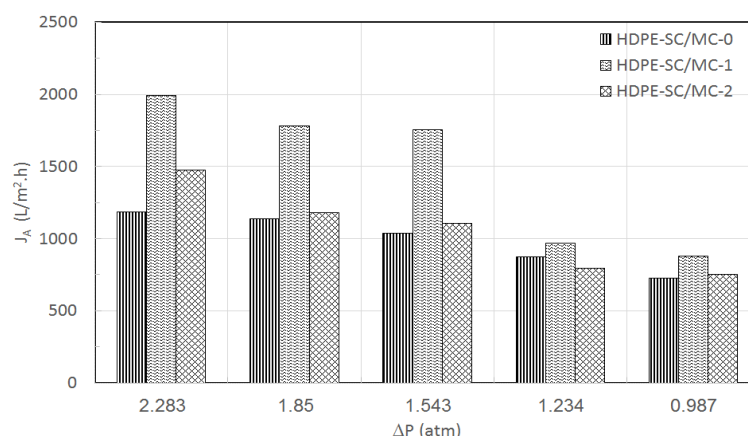
Figure 6. Effect of applied pressure on the membrane flux.
