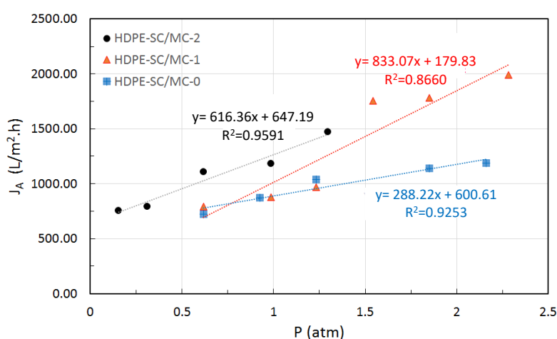
Figure 7. Pure water permeability of the obtained membranes.
