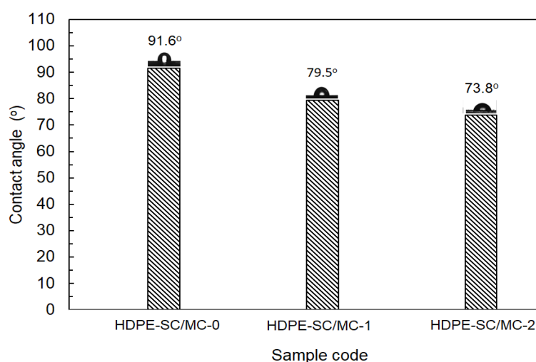
Figure 4. The images and contact angle values of the prepared mixed matrix membranes.
